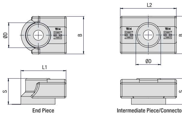
End Piece
