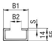
Mounting Rail TS-14
